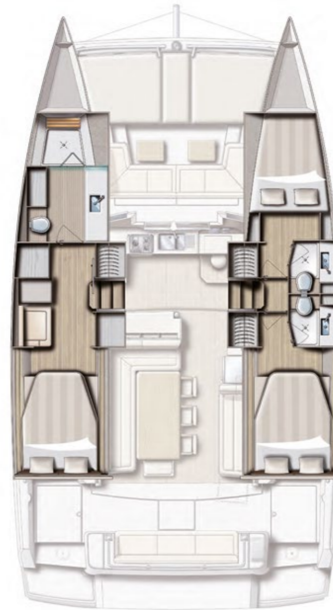
3 CABINS / 3 HEADS VERSION VERSION 3 CABINES / 3 SDB
