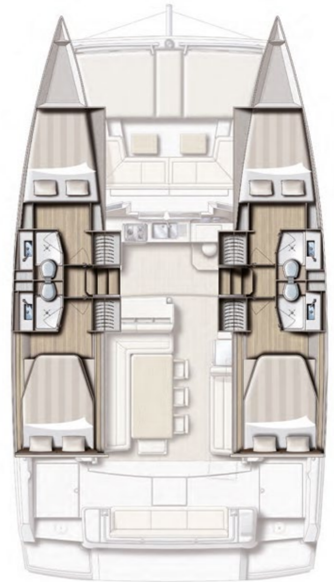
4 CABINS / 4 HEADS VERSION VERSION 4 CABINES / 4 SDB
